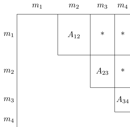
FIG. 2.4. Example of a nilpotent A in staircase form.
