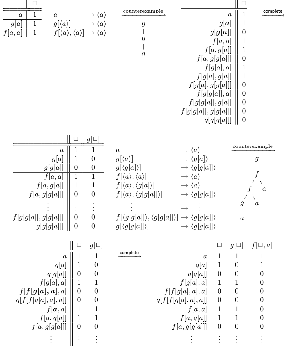
Figure 1: A run of L_*^{\text{fta}} , showing (partial) observation tables, inconsistencies (in boldface letters), transitions resulting from the rows of consistent tables (except for the final table), and counterexamples that the teacher may choose to return.
